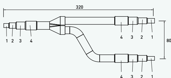
Liquid piping
