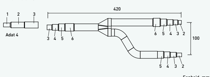
Liquid piping
